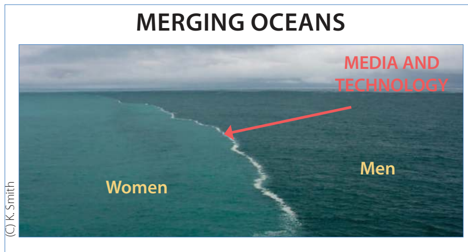
Figure 8 Merging Oceans
